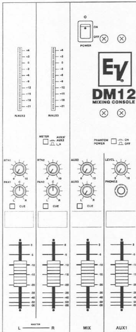
FIGURE 4 — DM Series Output Section Controls
